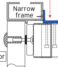
Angle Bracket (21020&21021)
