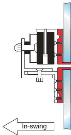
Bracket Kit for Mounting Mini Magnetic Lock on Full Glass Door and Frame. (21095N-In & 21095N-Out)
