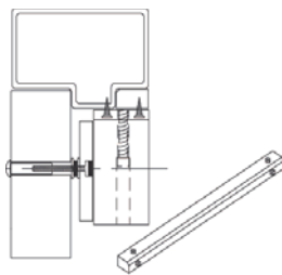
Filler Plate (21000 - 21005)
