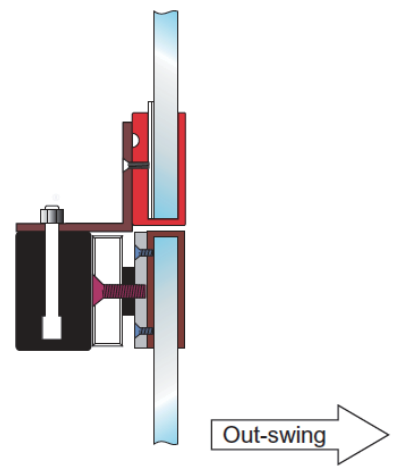
Bracket Kit for Mounting Mini Magnetic Lock on Full Glass Door and Frame. (21095N-In & 21095N-Out)
