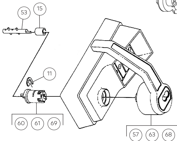
Right Hand Clutch
