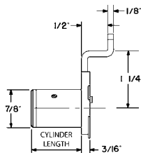
078-LB1-DW Installed Dimensions
