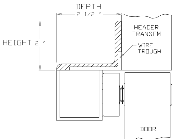
1194 ANGLE BRACKET
