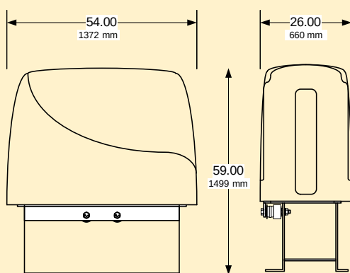
95xx-xxx with Standard Polyurethane housing
