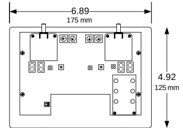
2372-080 Repeater
